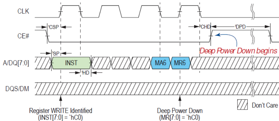
Figure 16: Deep Power Down Entry
