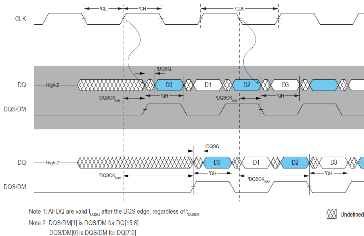
Figure 9: Read DQS/DM & DQ timing
