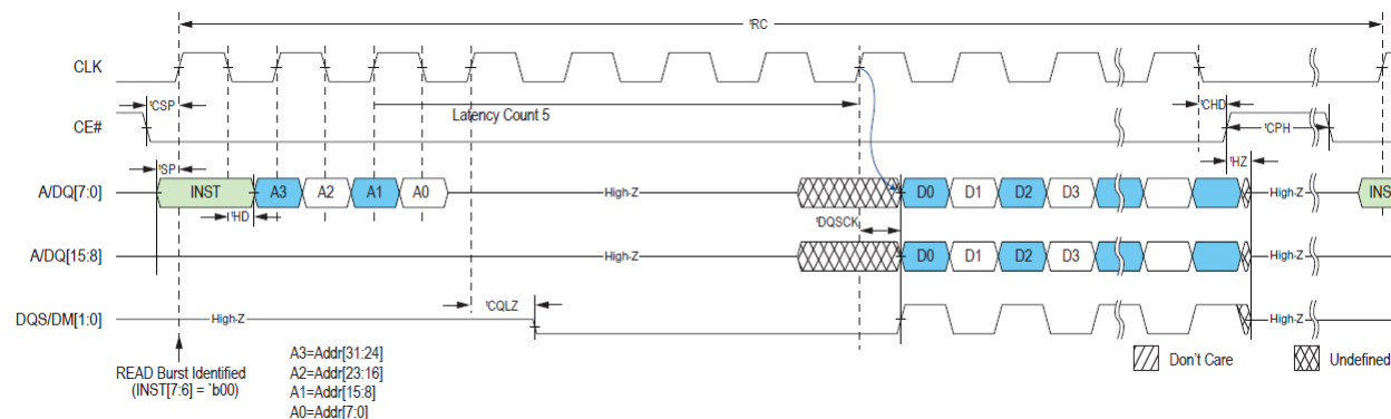
Figure 5: Synchronous Read
