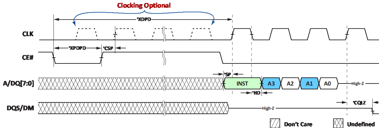
Figure 18: Deep Power Down Exit (Read Operation shown as example)
