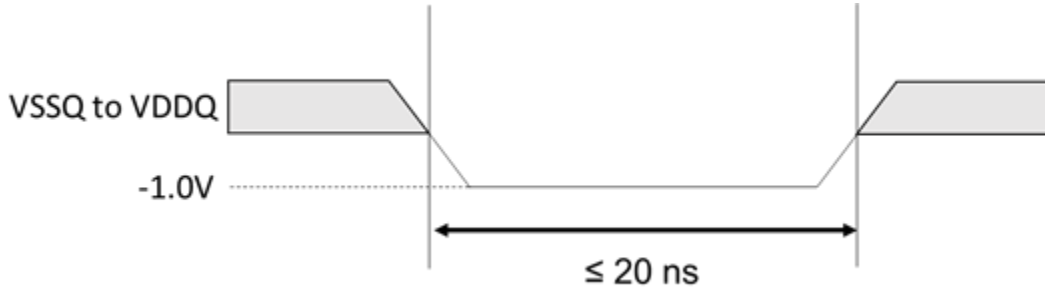
Figure 19 Maximum Negative Overshoot Waveform
