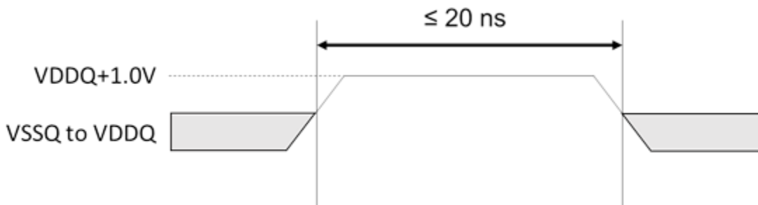
Figure 20 Maximum Positive Overshoot Waveform
