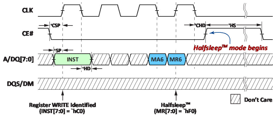
Figure 15: Halfsleep™ Entry Write (latency same as Register Writes, WL1)
