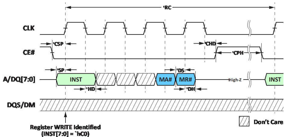
Figure 14: Register Write
