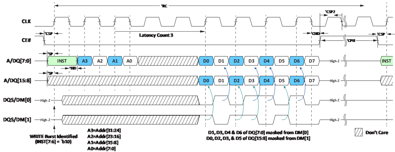
Figure 11: Synchronous Write followed by any Operation
