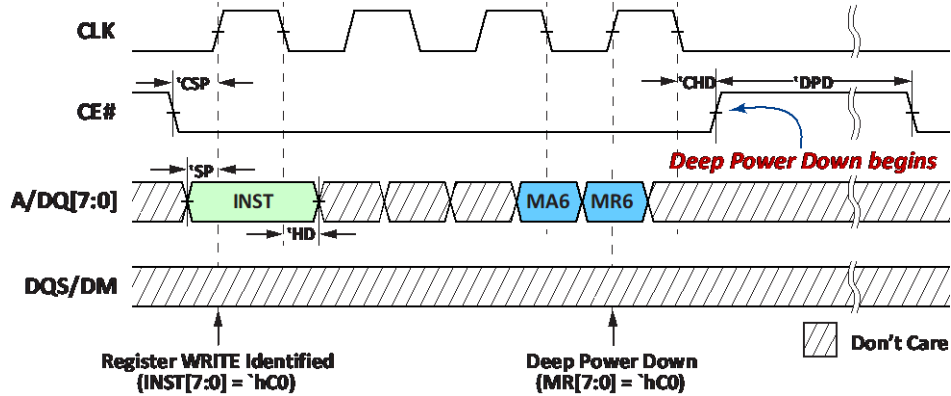
Figure 17: Deep Power Down Entry
