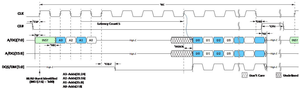
Figure 5: Synchronous Read
