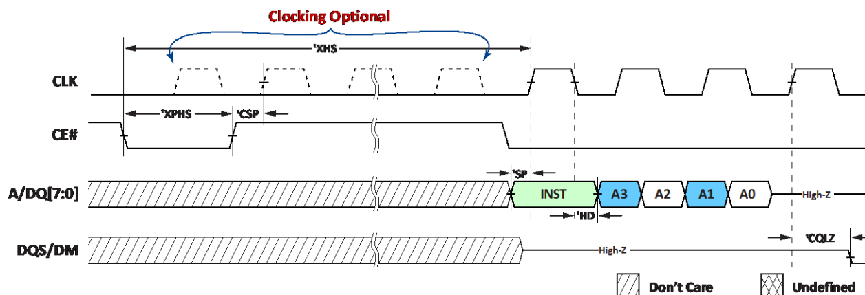
Figure 16: Halfsleep™ Exit (Read Operation shown as example)
