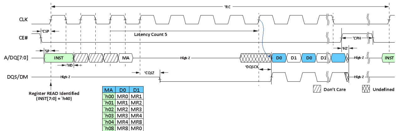
Figure 10: Register Read
