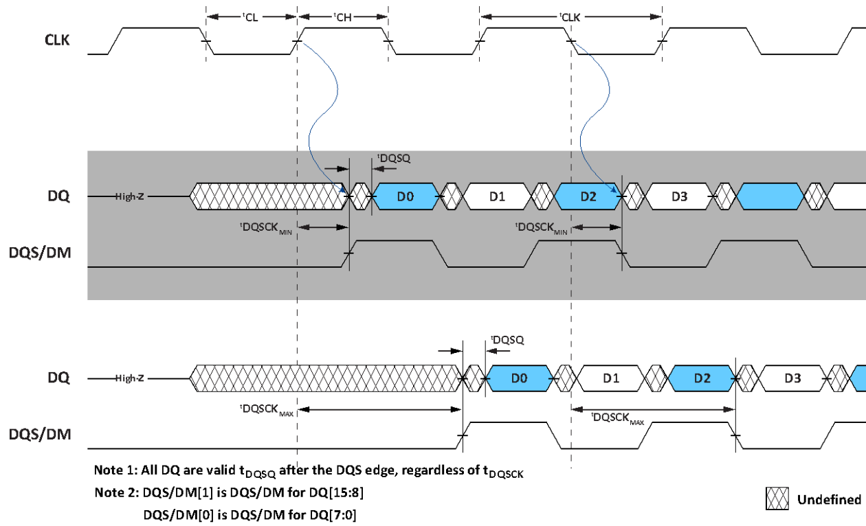
Figure 7: Read DQS/DM &amp; DQ timing
