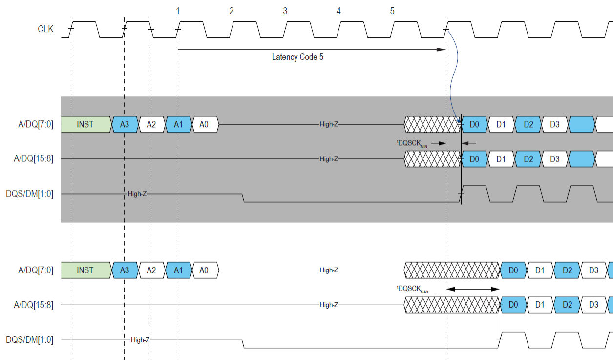
Figure 6: Read Latency & tDQSK
