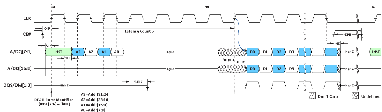
Figure 3: Synchronous Read
